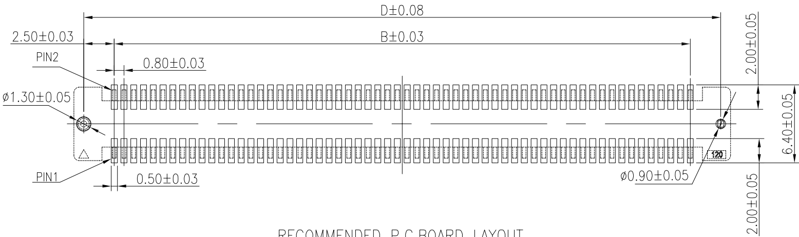
RECOMMENDED P.C.BOARD LAYOUT
